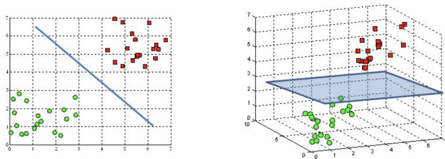
Figure 2: A hyperplane in 2D is a line; a hyperplane in 3D is a plane.
